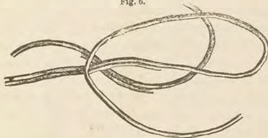
PALÆOCHORDA MINOR. (One half nat. size.)
